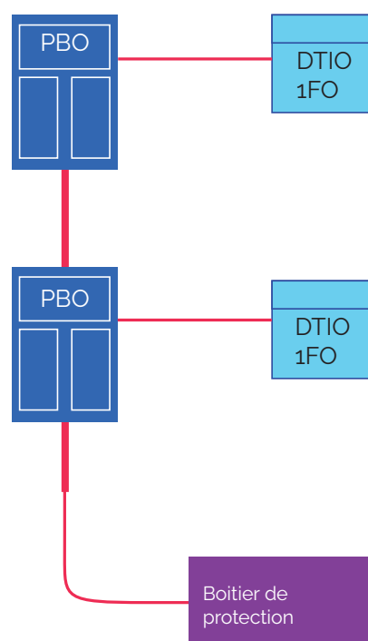
Fig. 08 | Architecture mono-fibre
