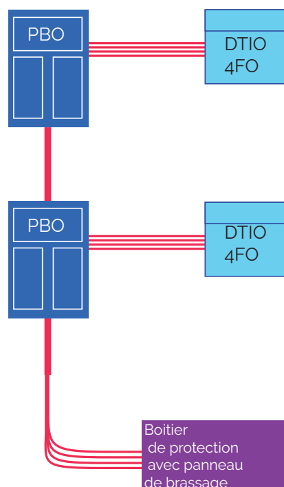
Fig. 09 | Architecture quadri-fibre
